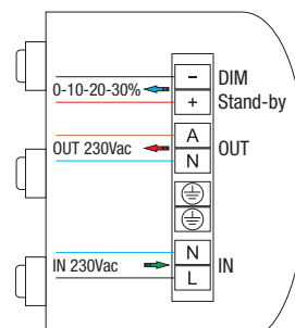
Schema collegamento - Wiring diagram
