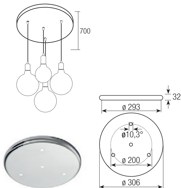
ROSONE TONDO Ø 305 - 4 FORI ROUND CEILING ROSE Ø 305 - 4 HOLES
