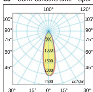
30° - Semi-concentrante - Spot
