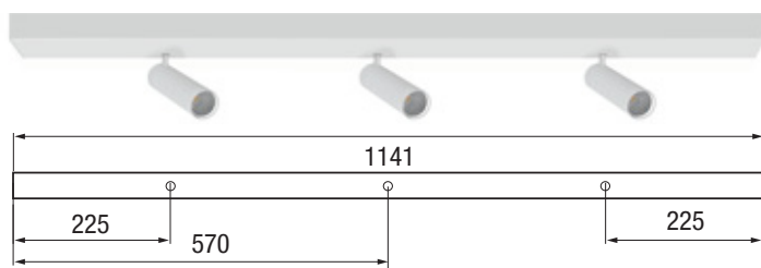
Spot 15°
